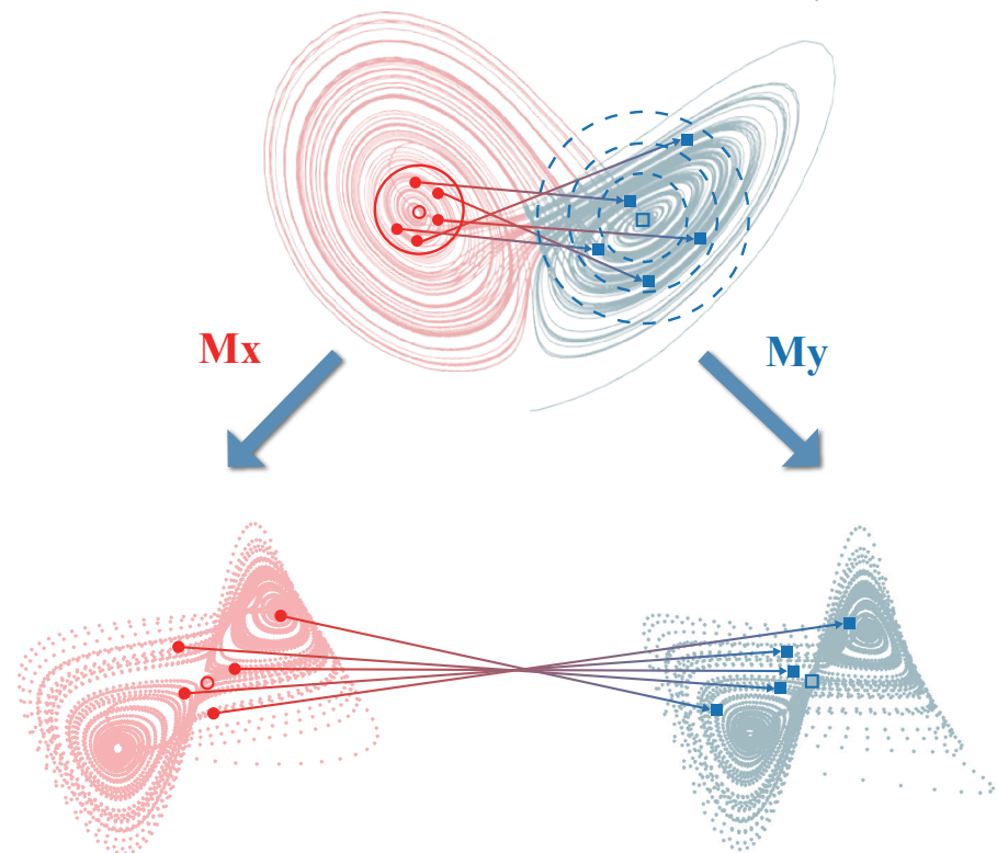
b. Intersectional cardinality ( H_0 )
